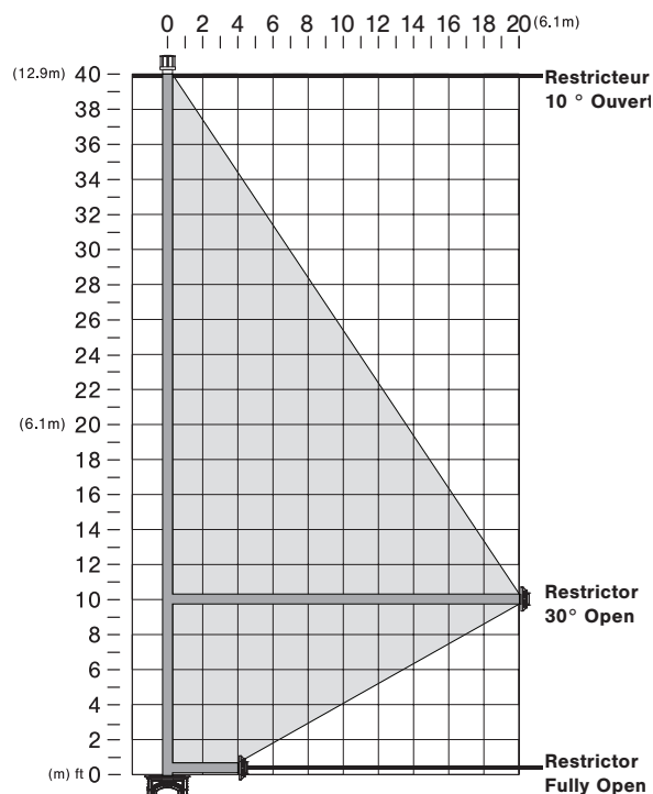
NG/LPG - TOP VENT COMBINATION VENTING (V/H)
