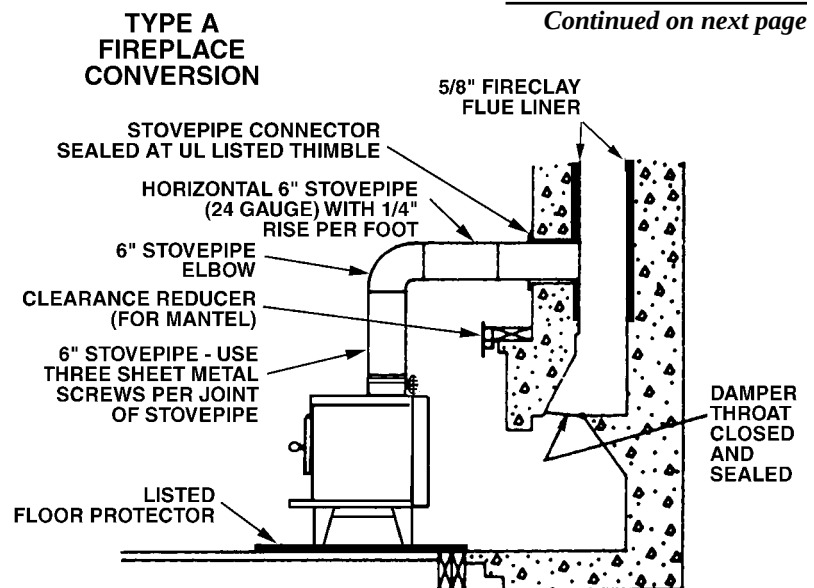
FIG. 10 - Fireplace Conversion
