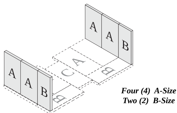
Fig.4b– Step 2, Side Firebrick Installation
