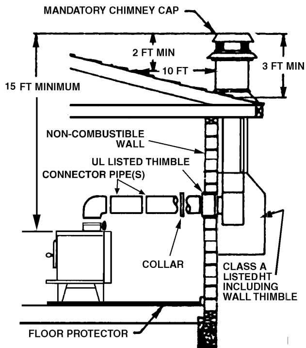
Fig. 9 - Chimney Connection to Firebox Through Masonry Wall
