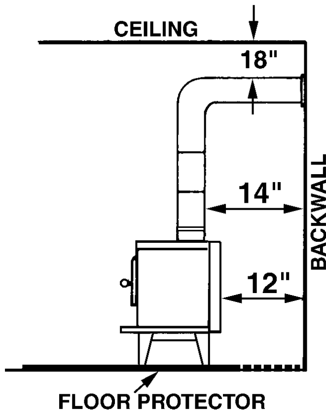
Fig. 3b – Side View Minimum Clearance Dimensions from Combustible Surfaces
