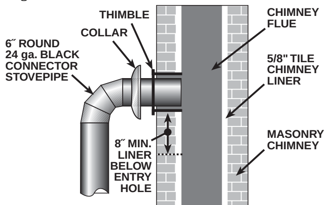
Fig.6 - Masonry Chimney Connection
