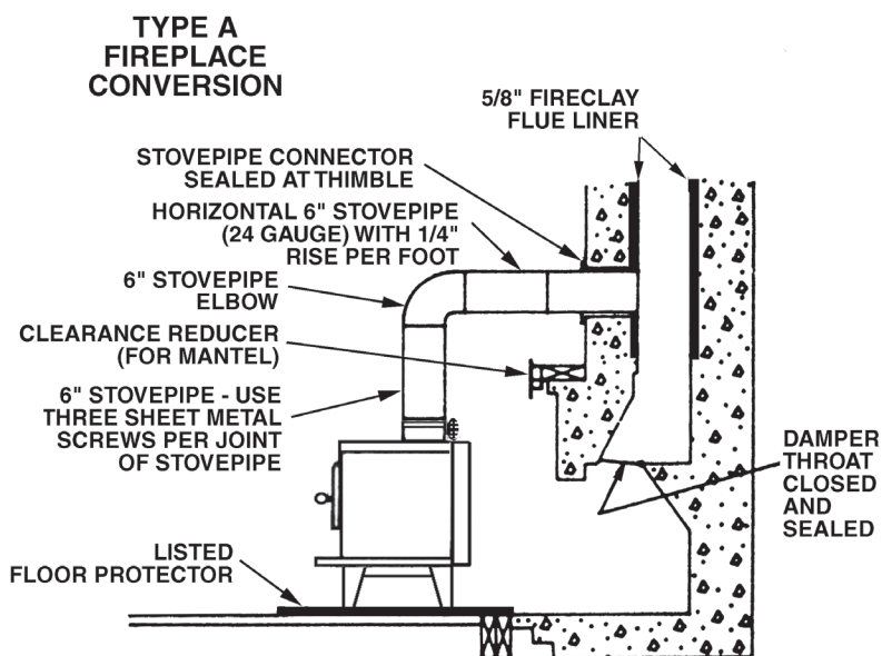
Figure 19 - Fireplace Conversion
