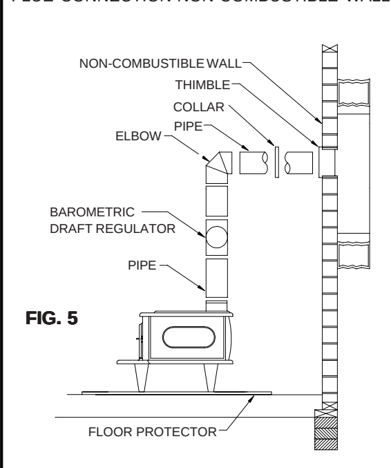
FLUE CONNECTION-NON-COMBUSTIBLE WALL
