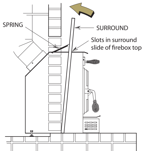
Figure 6. Surround Installation
