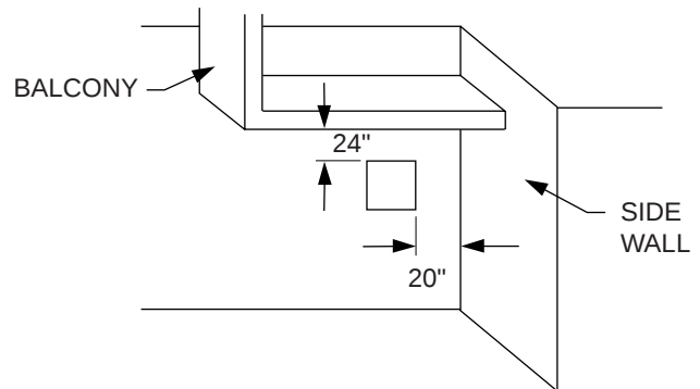
BALCONY WITH PERPENDICULAR SIDE WALL
