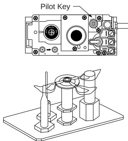
Fig. 10 - Pilot flame adjustment
