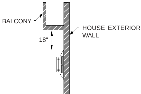
BALCONY - NO SIDE WALL (CROSS SECTION)
