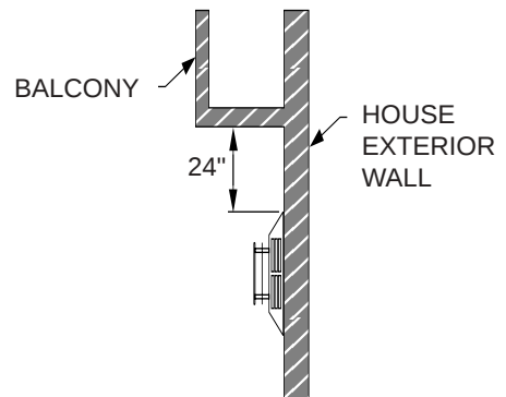
BALCONY - NO SIDE WALL (CROSS SECTION)
