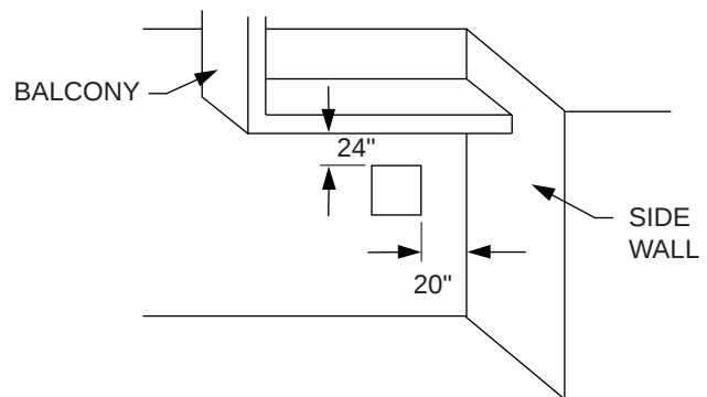
BALCONY WITH PERPENDICULAR SIDE WALL
