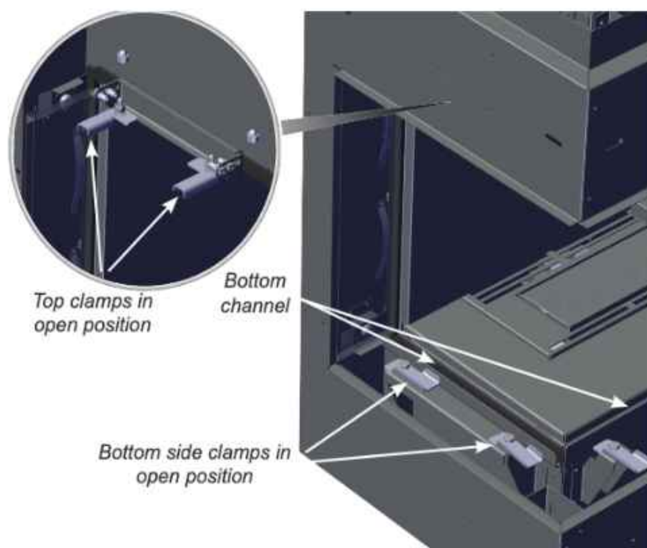
CC40LE/CC40RE shown
