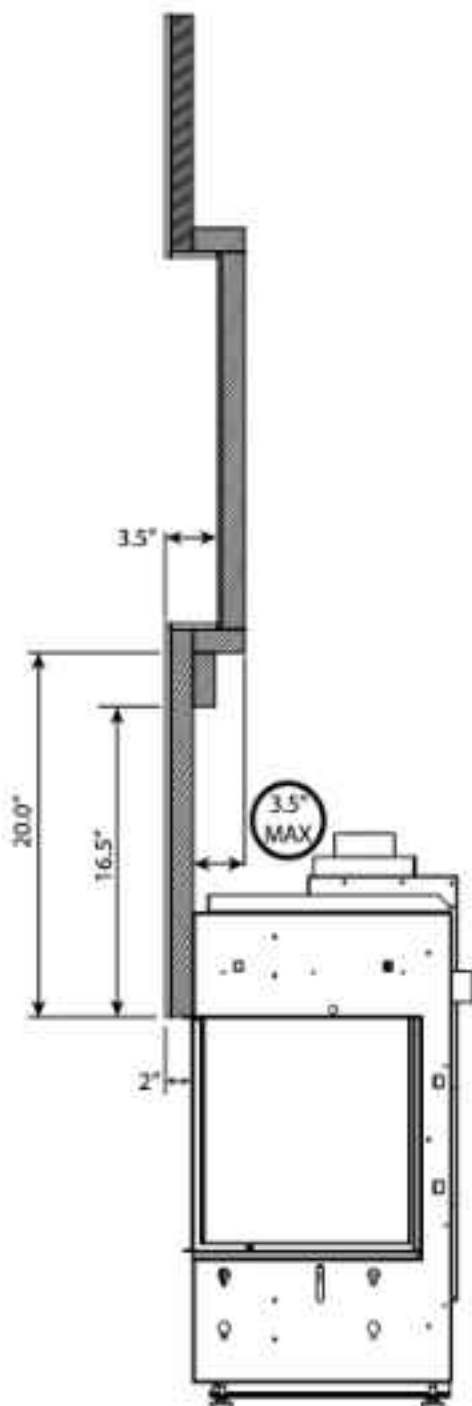
Sample Install 1
