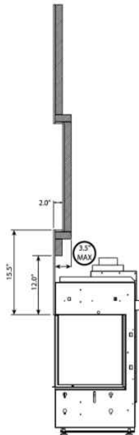
Sample Install 2
