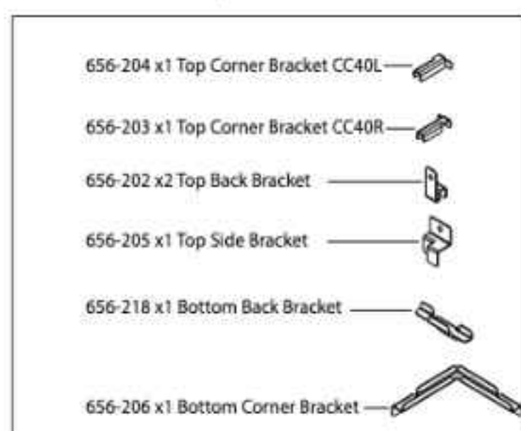
Glass Panel Parts Layout
