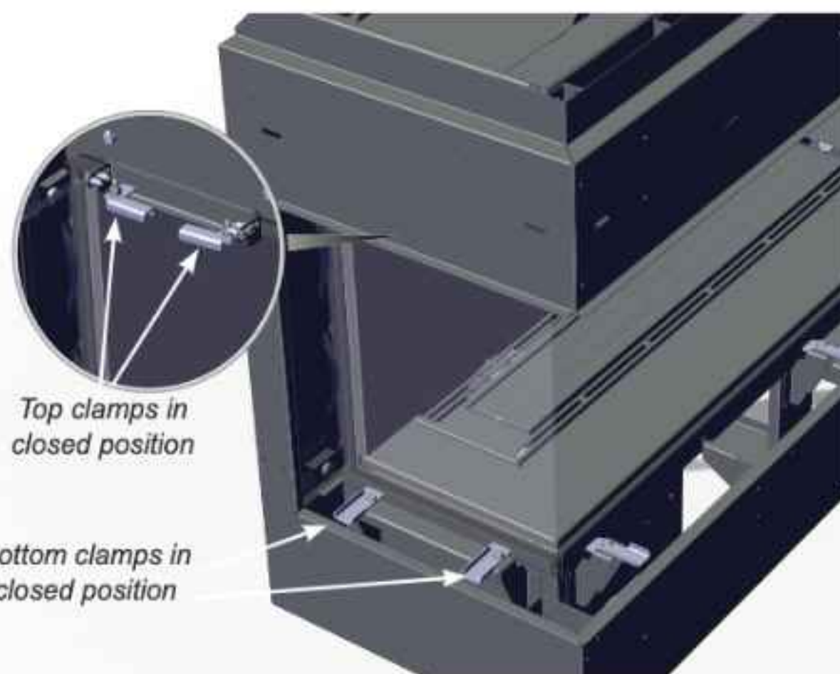
CC40LE/CC40RE shown
