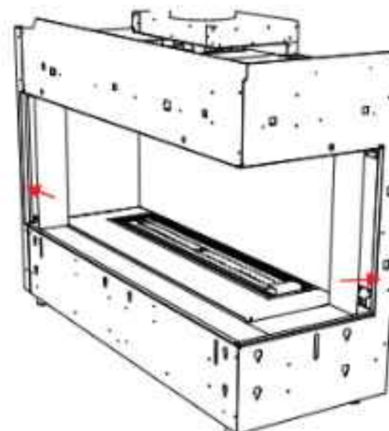
Outer side panel install
