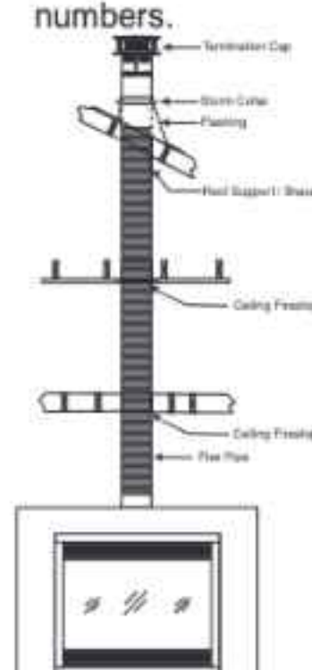
Diagram 3
