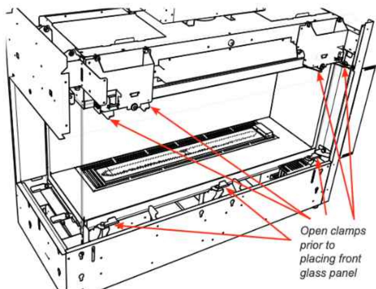
CC40LE shown
