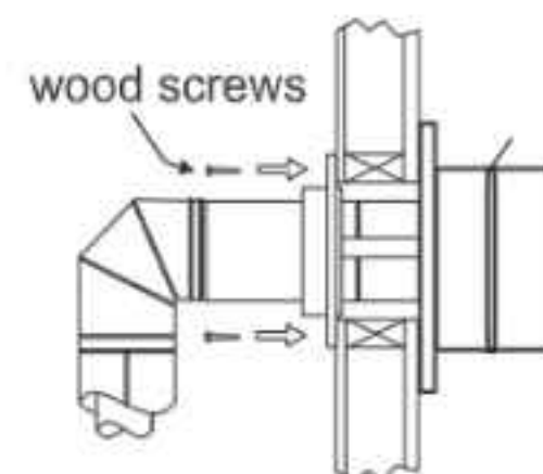
Diagram 4
