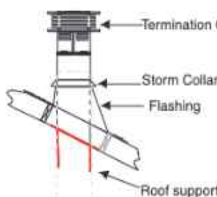
Diagram 3b
