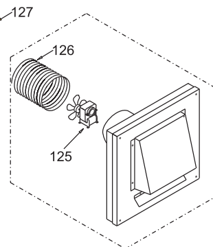
HEAT RELEASE DUCT KIT
