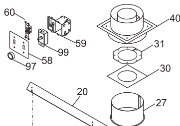
Top Nailing Strip Installation
