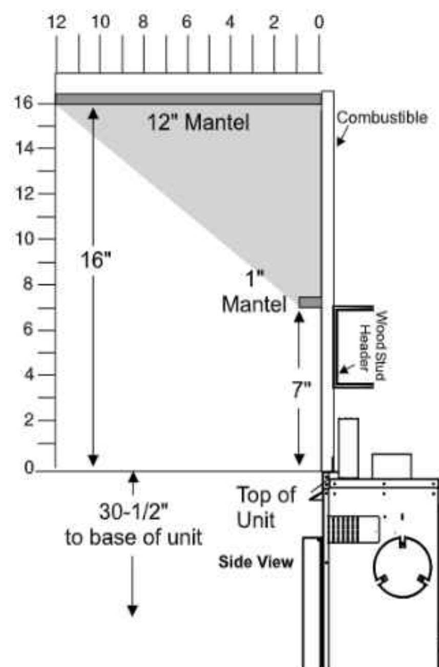
MANTEL CLEARANCES WITH SAFETY SCREEN AND LOUVERS
