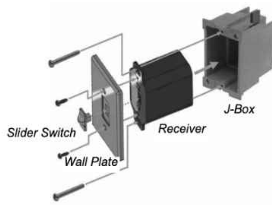
Low Voltage Junction Box
