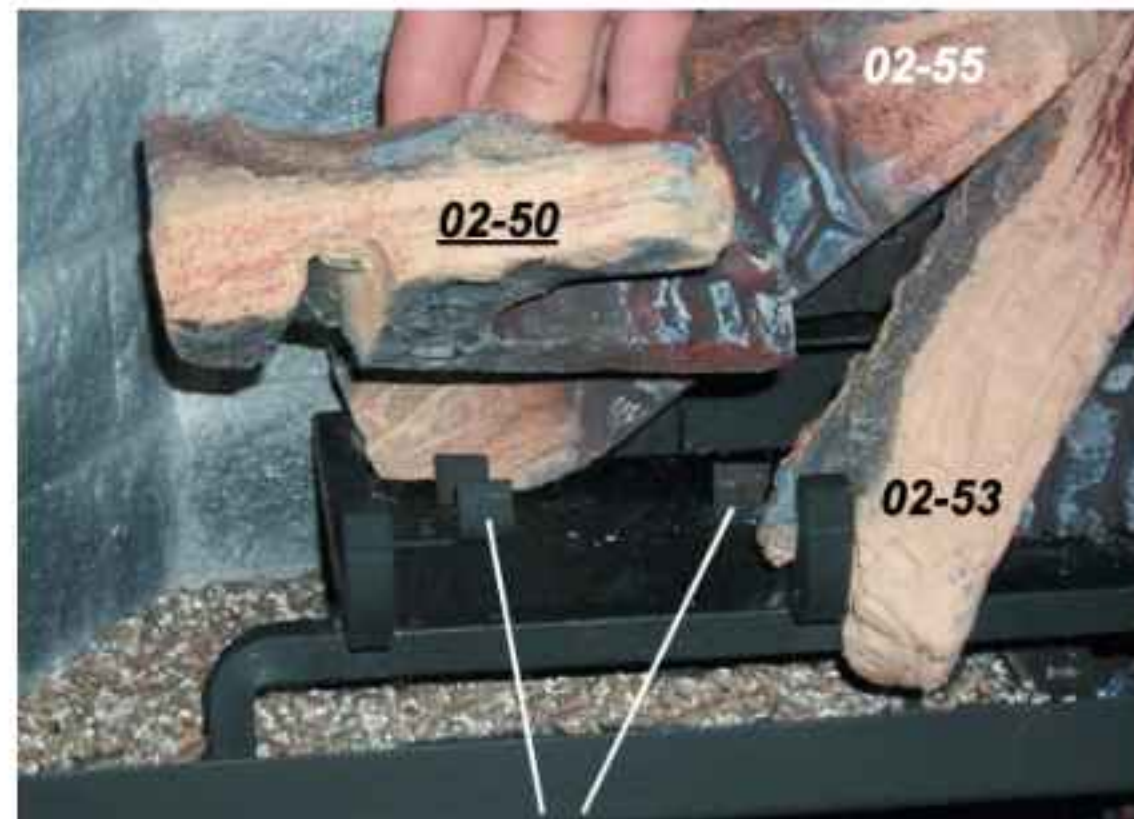
Front Brackets
