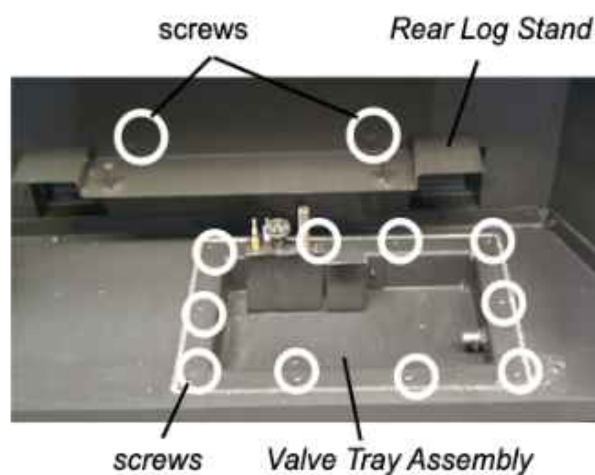
Diagram 2: Rear Log Stand and Valve Tray Assembly
