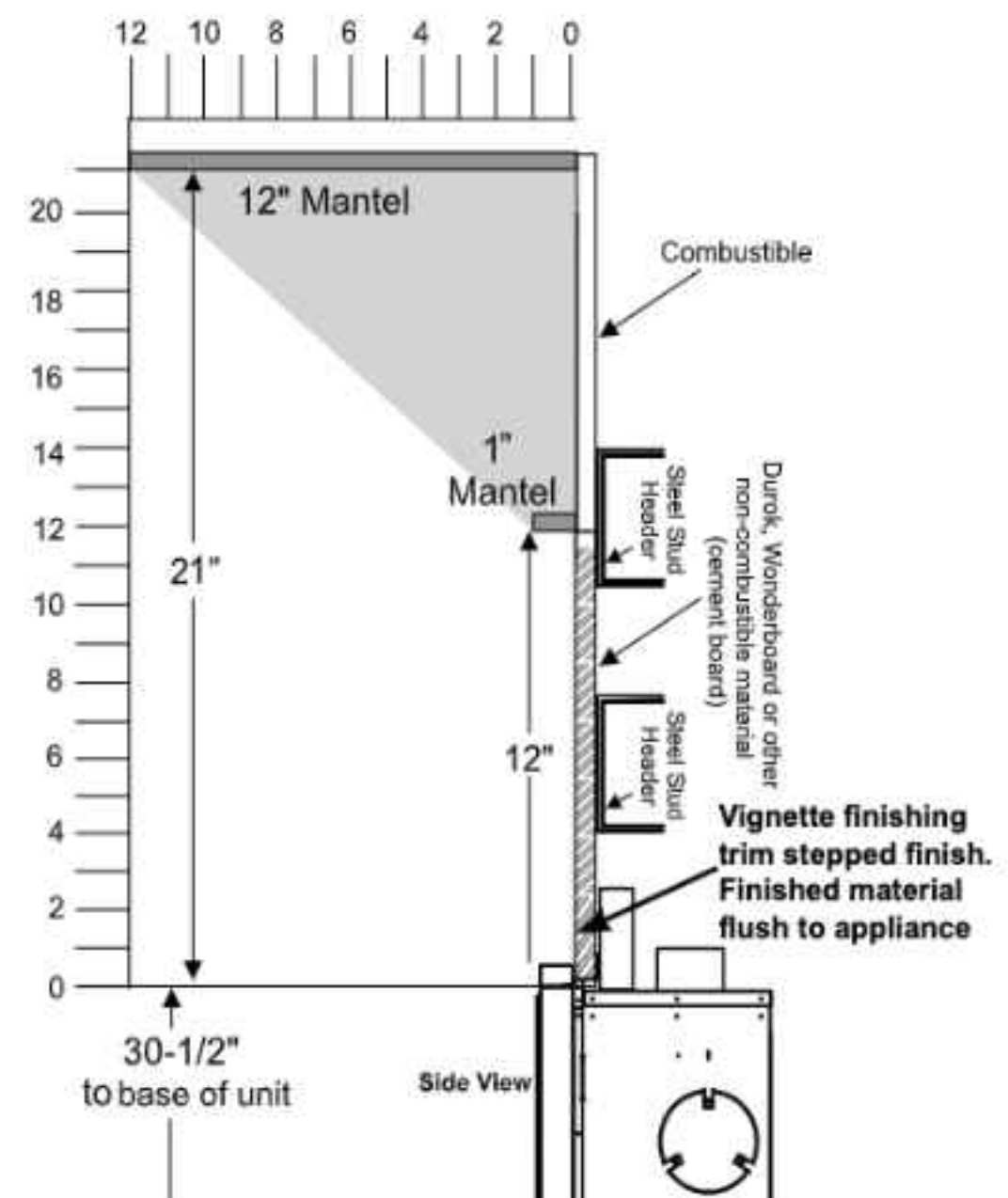
MANTEL CLEARANCES WITH SAFETY SCREEN AND LOUVERS
