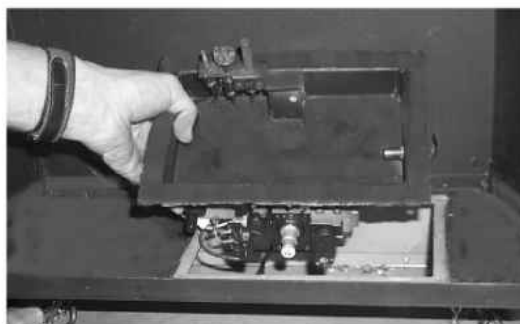
Diagram 3: Lift out Valve Tray Assembly
