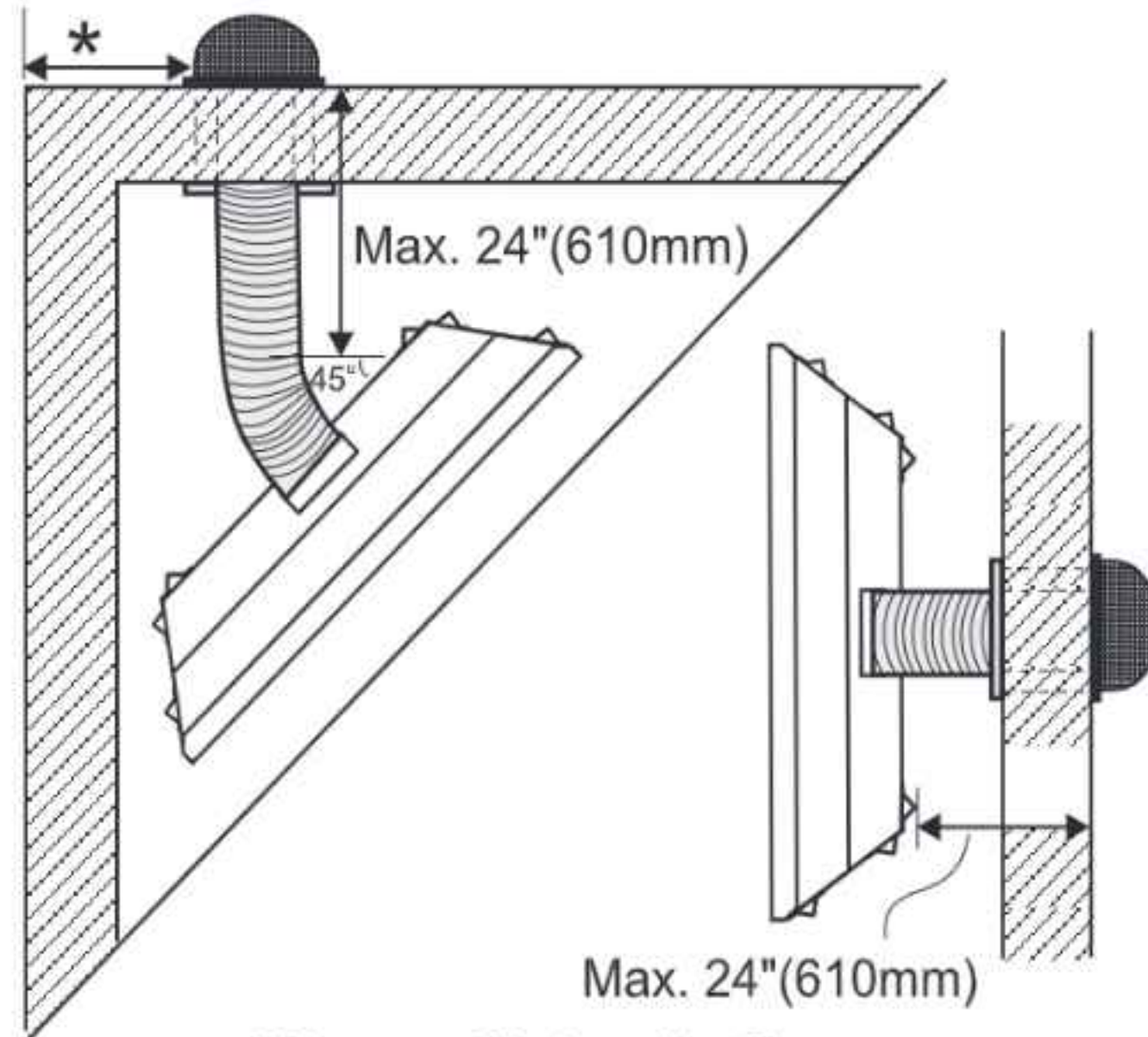
Minimum and Maximum Vent Clearances
