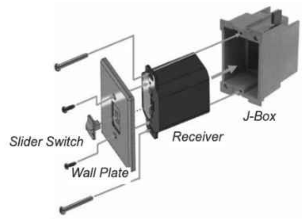
Low Voltage Junction Box
