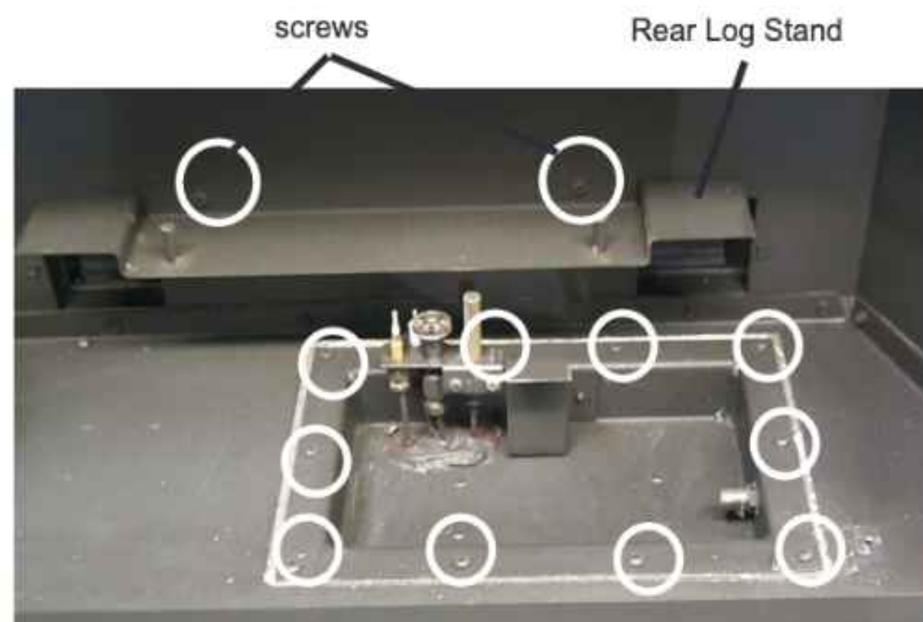
Diagram 2: Rear Log Stand & Valve Tray Assembly
