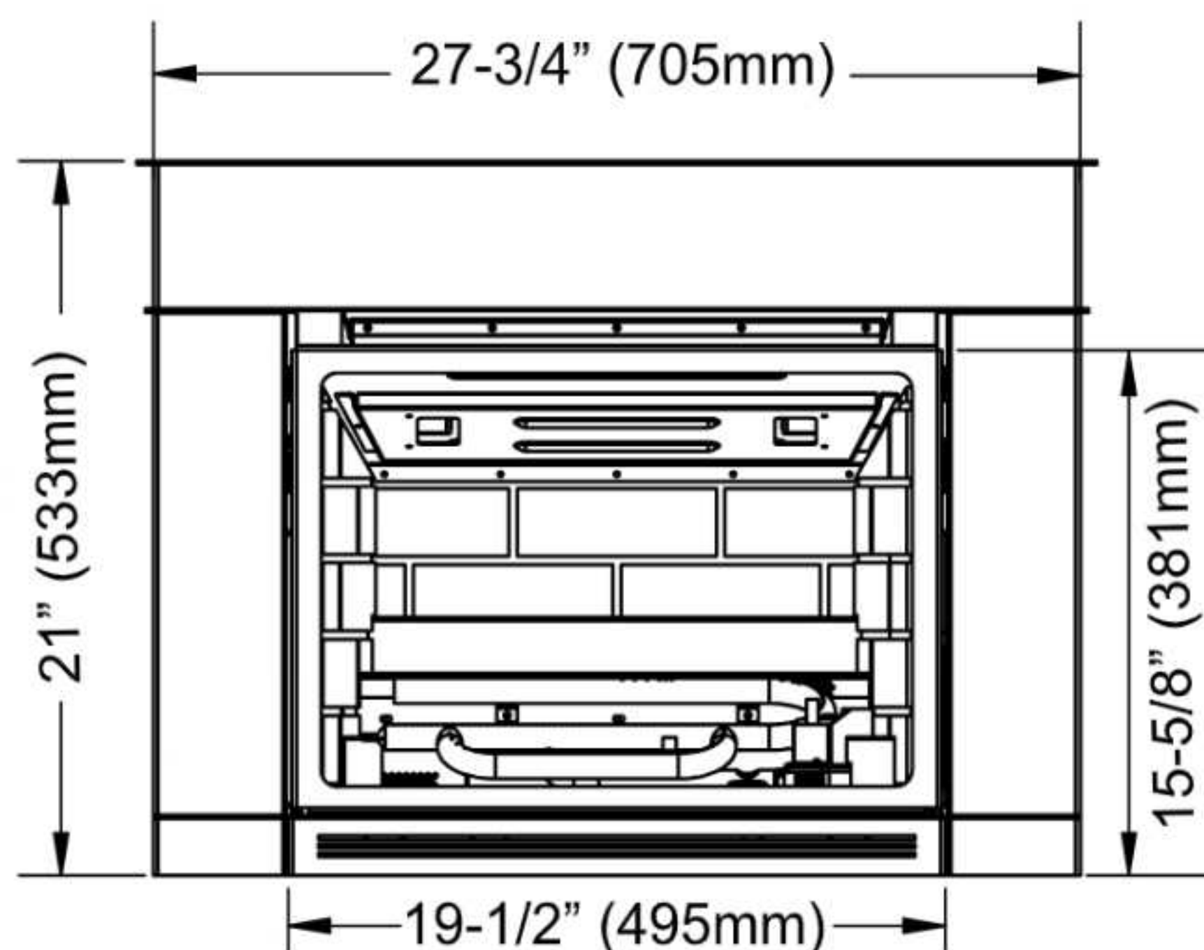
Contemporary Faceplate
