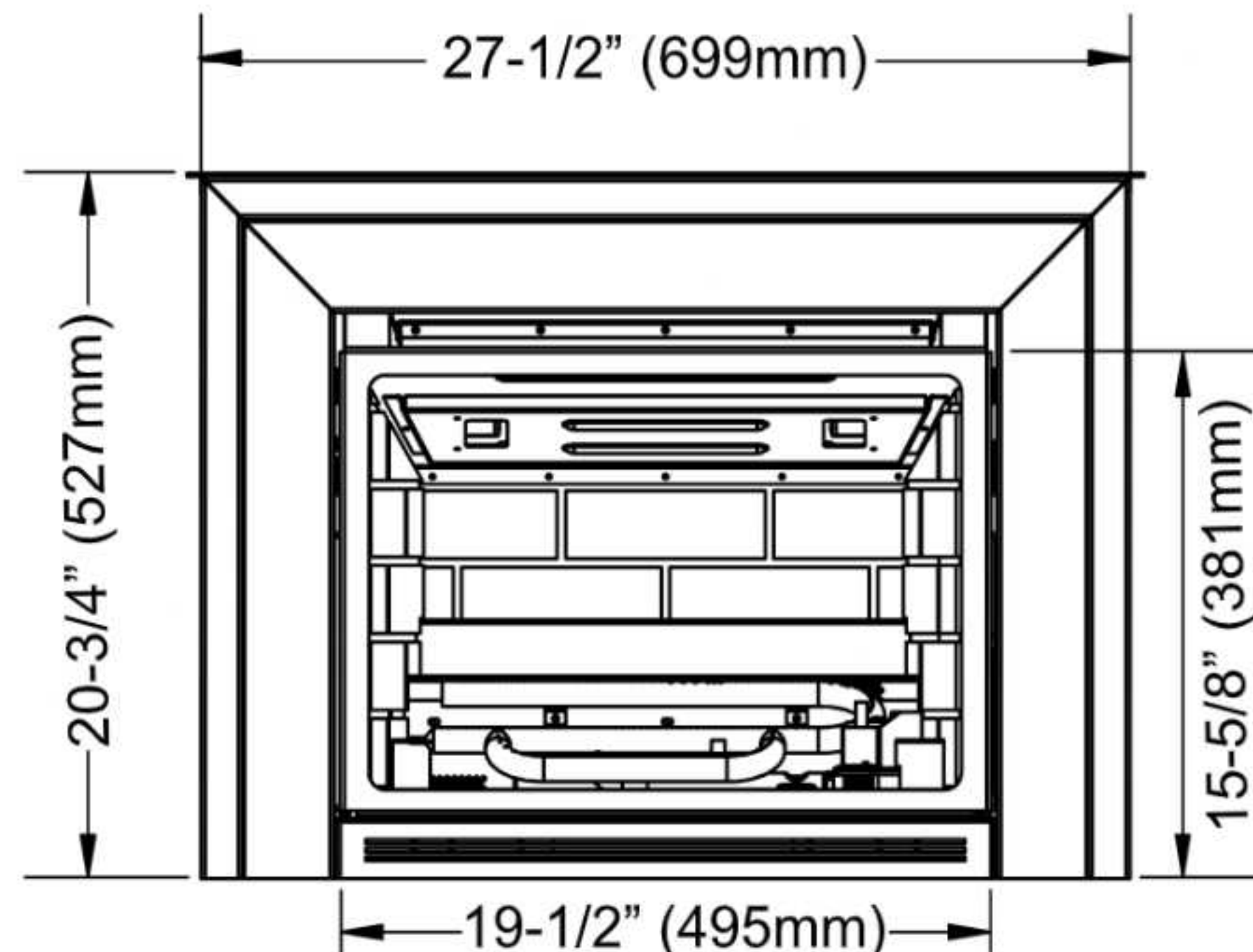
Contour Faceplate
