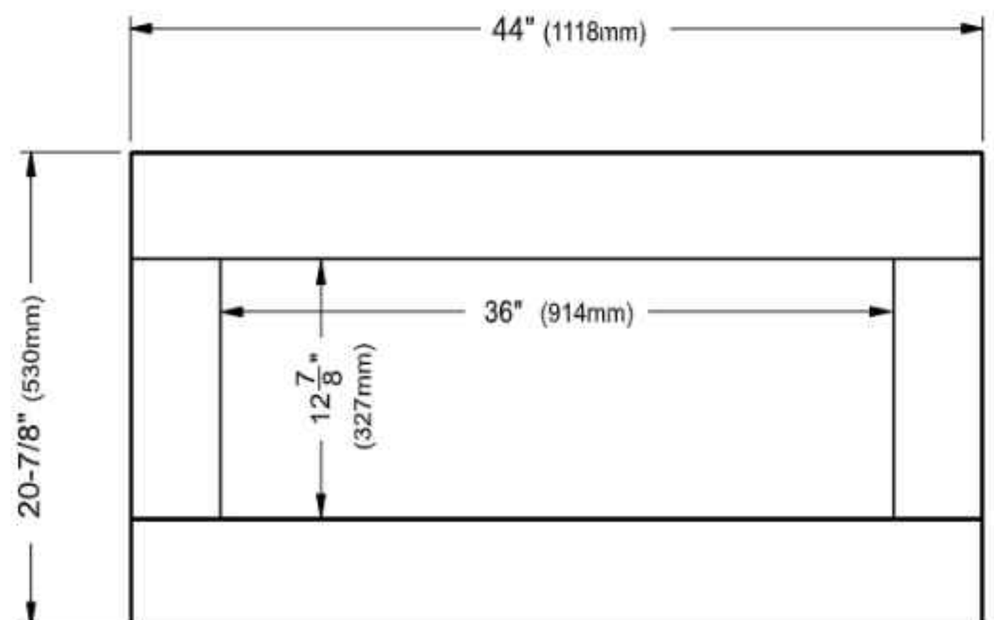
4 Piece Faceplate/Verona Surround
