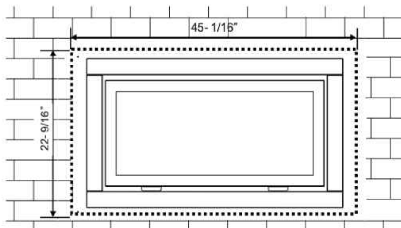
Unit shown with inner and outer door frame
