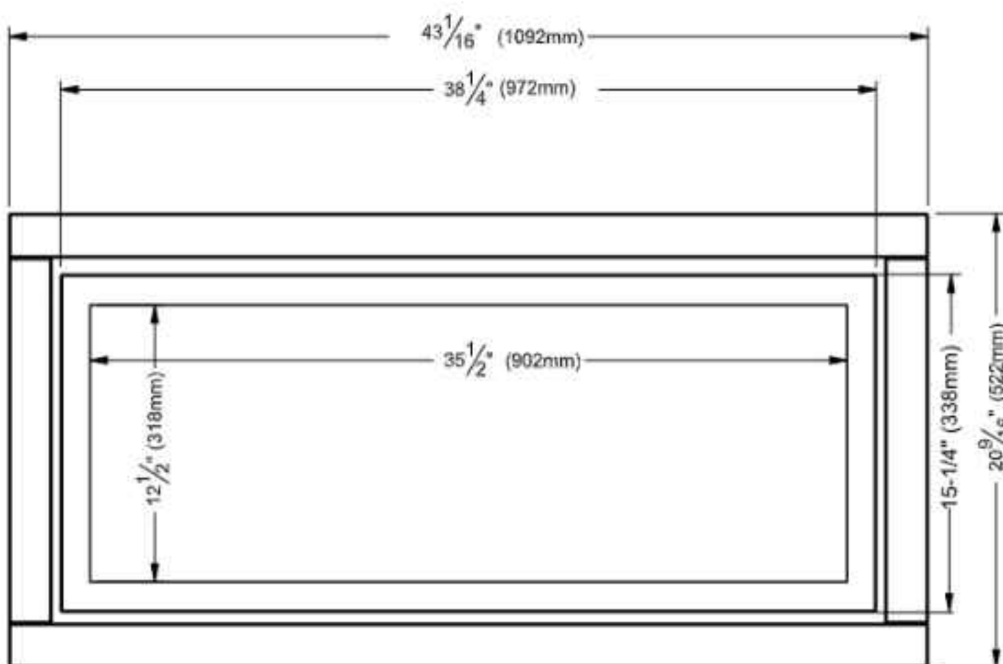
Inner/Outer Faceplate
