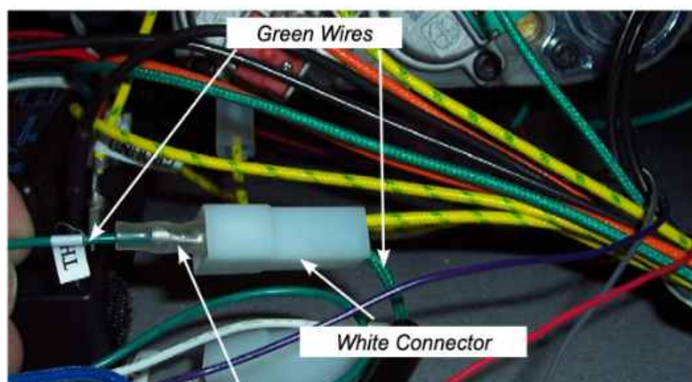
Disconnect green TH wire
