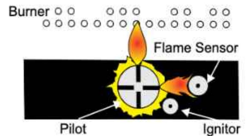
Top View of Pilot Flame
