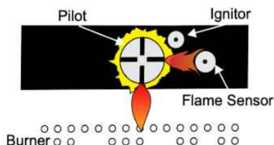
Top View of Pilot Flame
