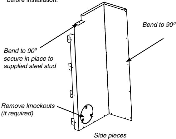
Framed opening - Side View
