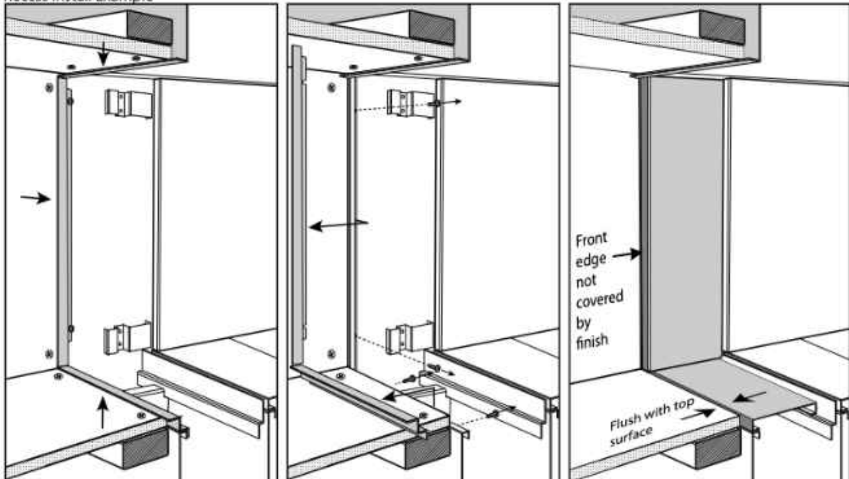
Recess Install Example
