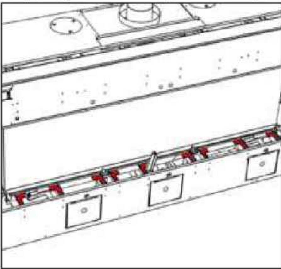
Lower clamps (x9) in open position
