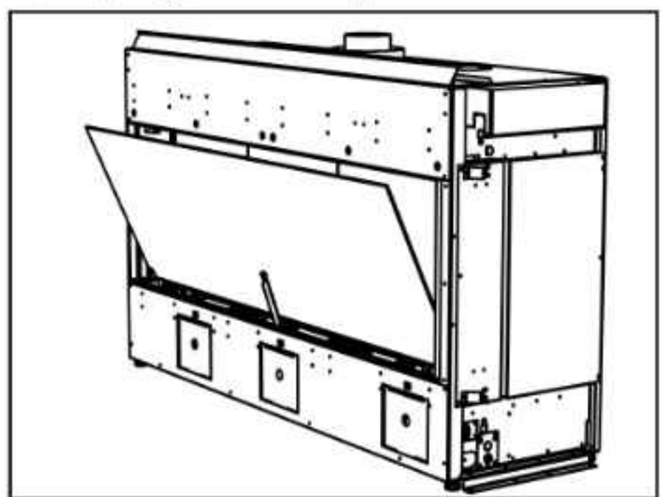
Glass panel--leaning on support
