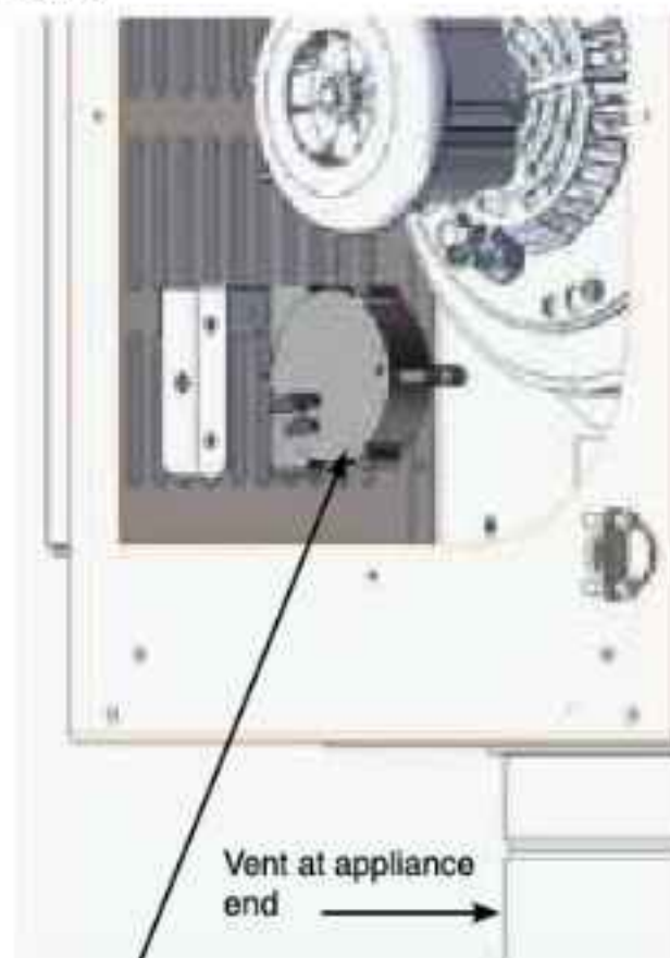
Pressure switch orientation if inline power vent is oriented vertically (see Diagram 1)
