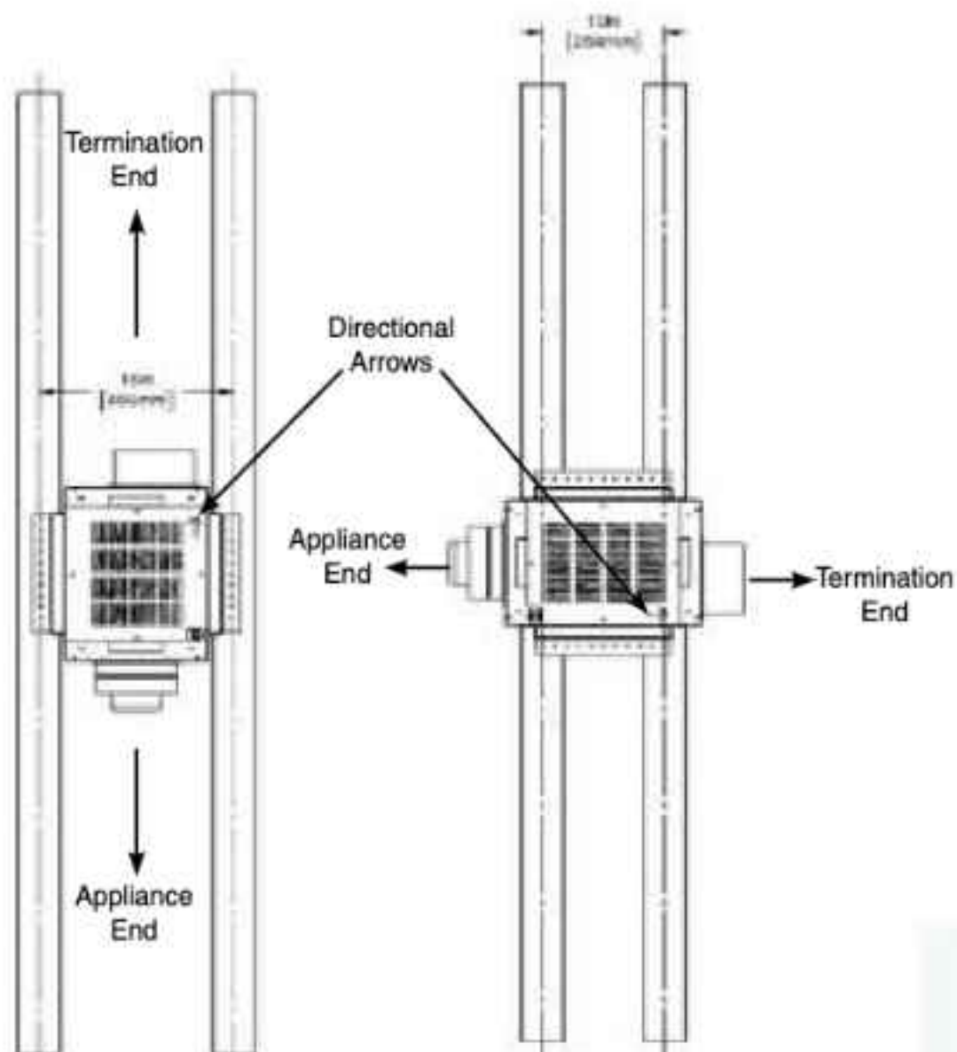
Diagram 1: Inline power vent oriented vertically
