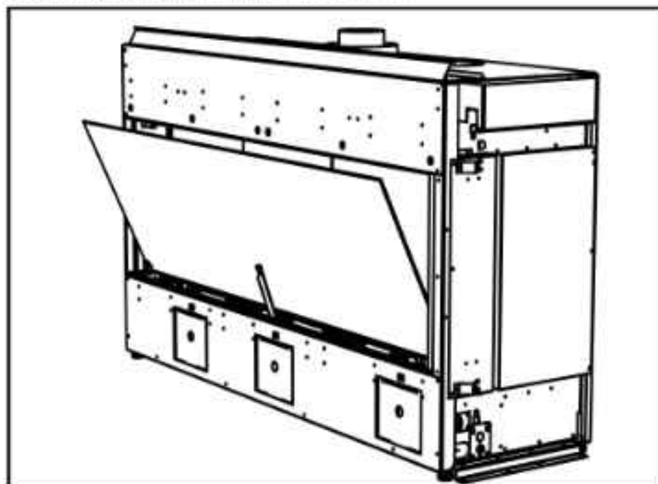
Glass panel--leaning on support
