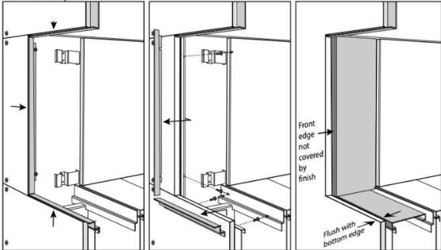
Flush Install Example
