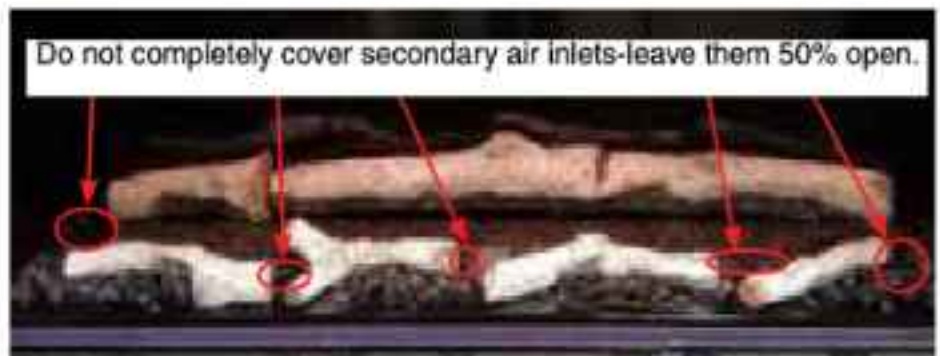
Correct Black Coal placement
