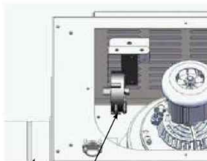
Pressure switch orientation if inline power vent is oriented vertically (see Diagram 1)
