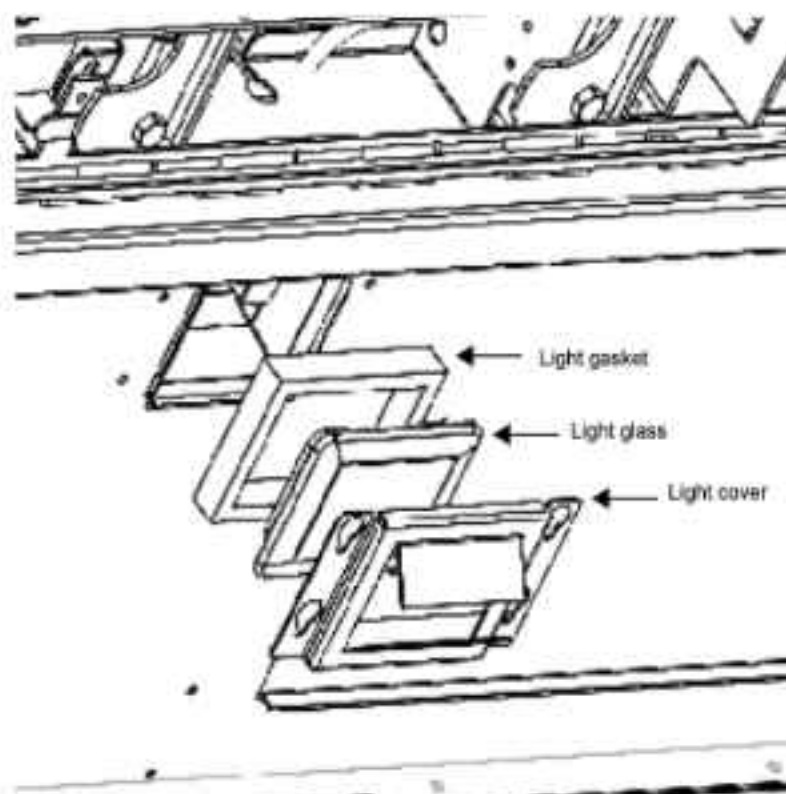
Inner light cover reassembly order
