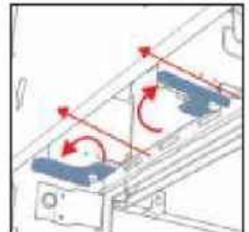
Clamps in open position, rail pulled forward
