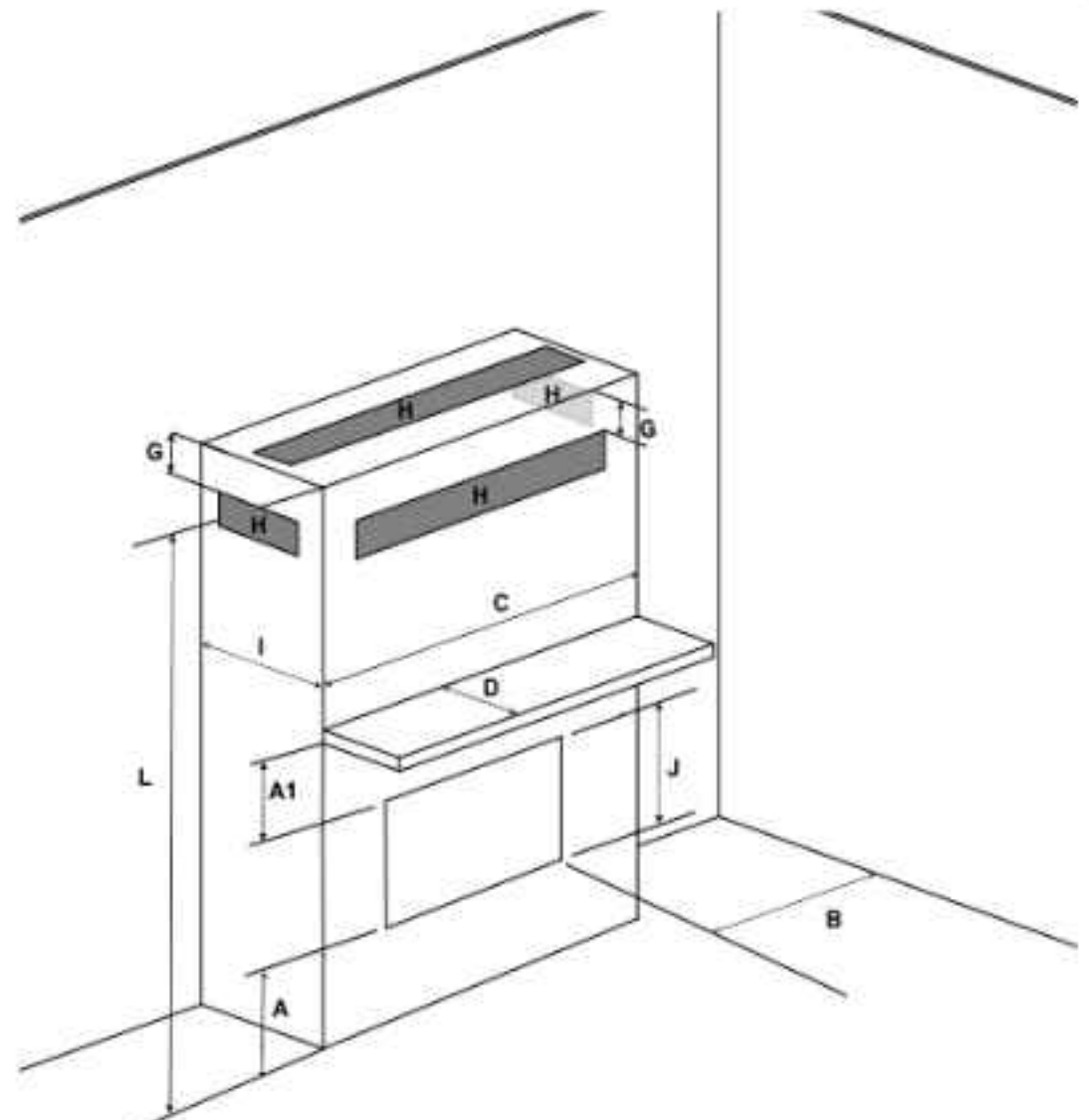
Low framing with ventilation opening in front/2 sides or top
