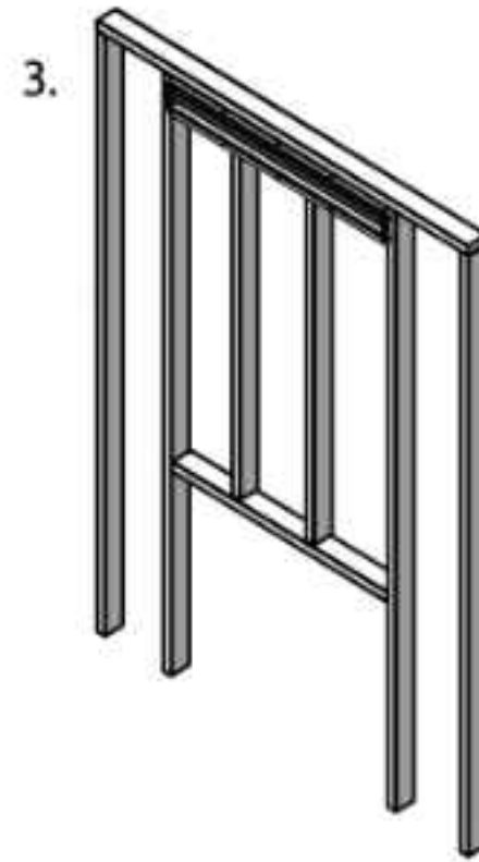
Use at least 3 sets of screws to keep the vent flat against framing
