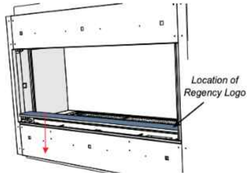
Outer front panel install
