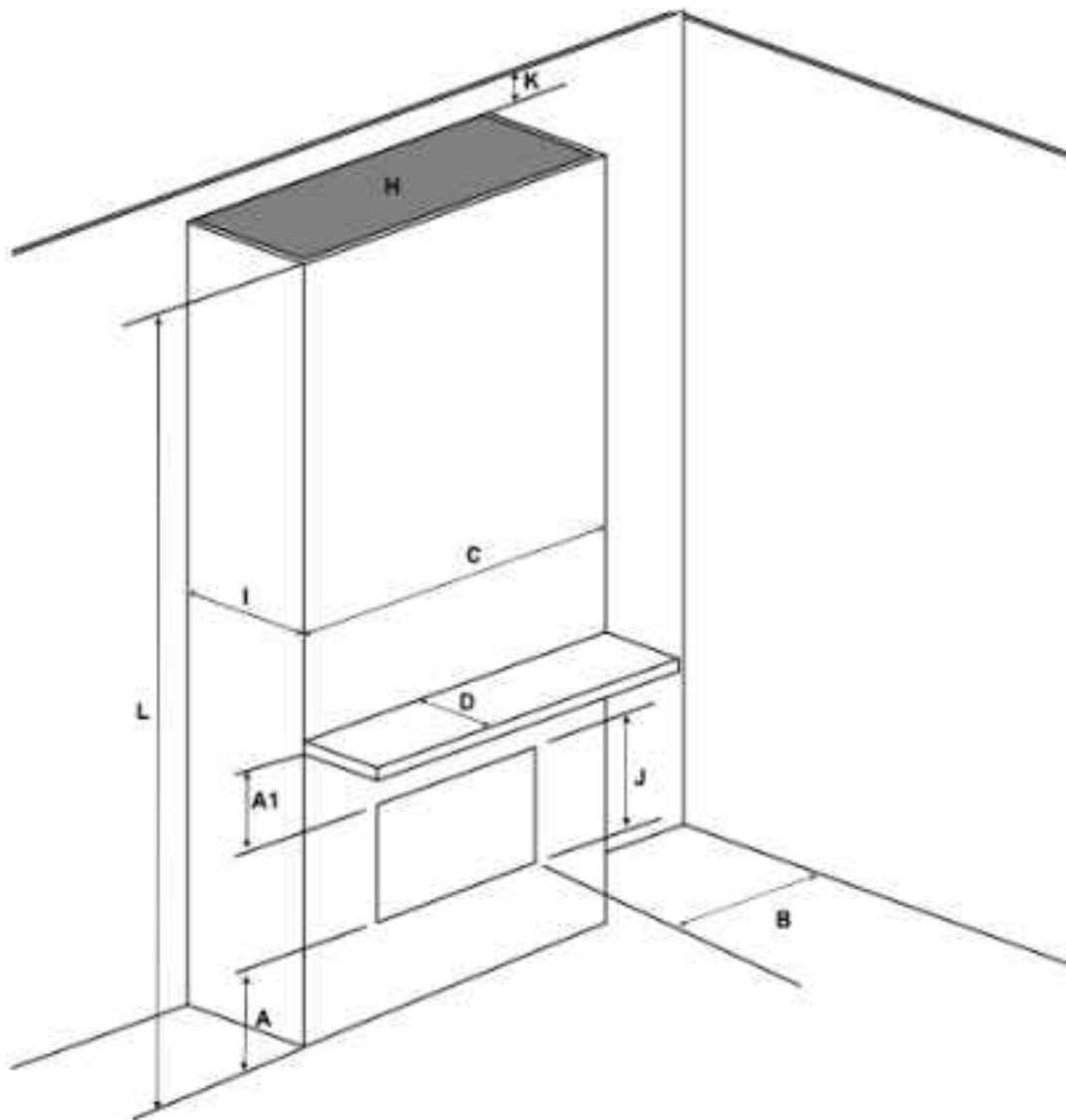
Floor to ceiling with top ventilation opening
