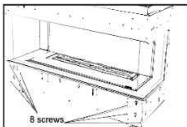
CB40EPV screw locations
