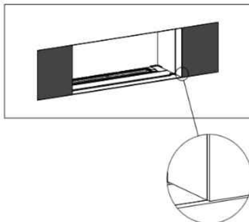
Correctly installed glass panels
