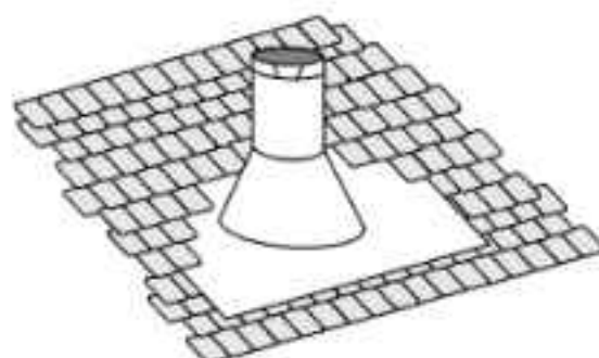
Diagram 4 - The upper half of the flashing is installed under the roofing material and not nailed down until the chimney is installed, to allow for small adjustments.
