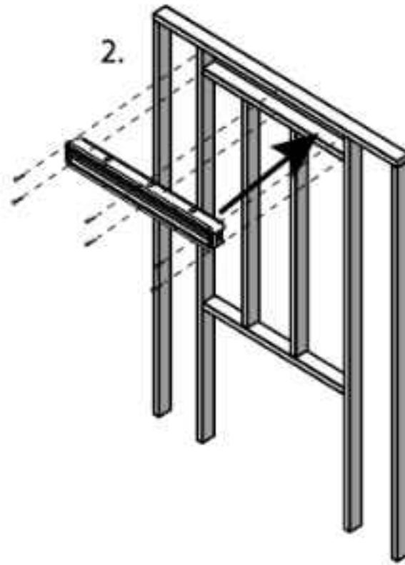
Screw Chase vent to Framing
