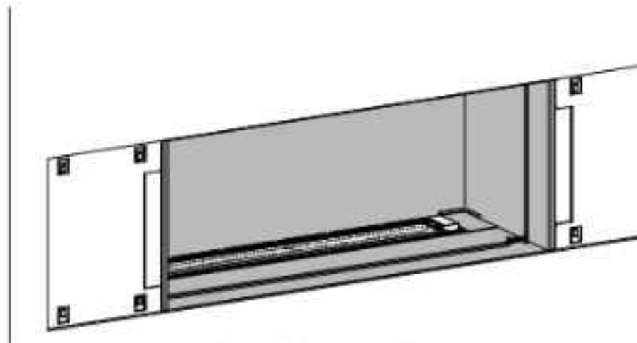
Install inner panels
