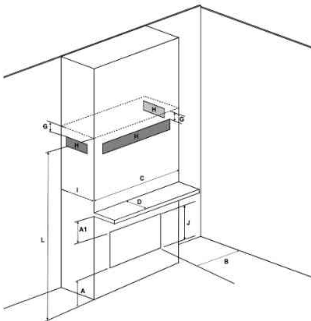
Full framing with low ventilation opening in front or 2 sides
