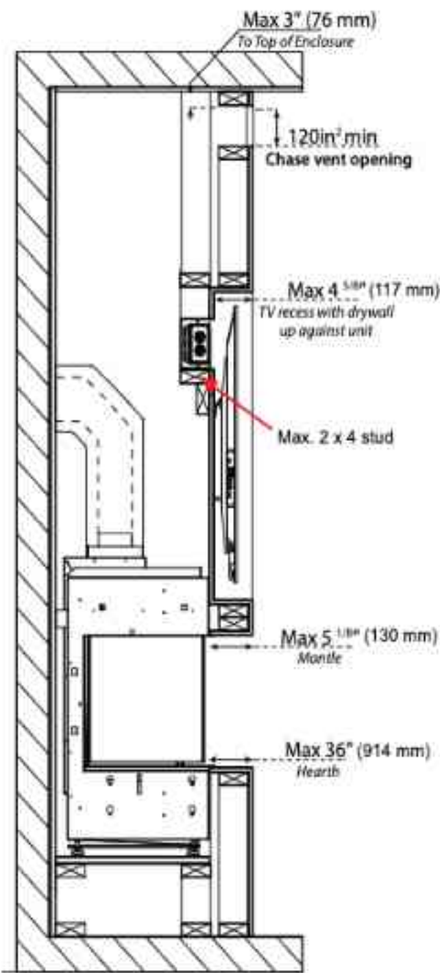
4 5/8" (117 mm) maximum TV recess using 1/2" (13 mm) drywall
