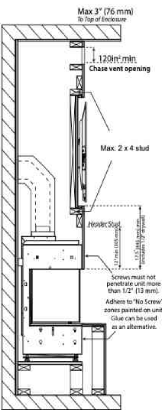
Flush wall TV recess using 1/2" (13 mm) drywall
