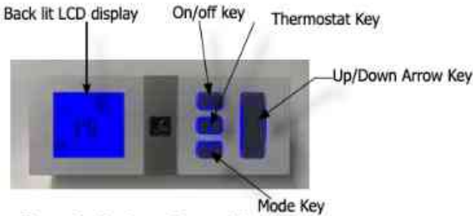
Figure 2: Proflame Transmitter
