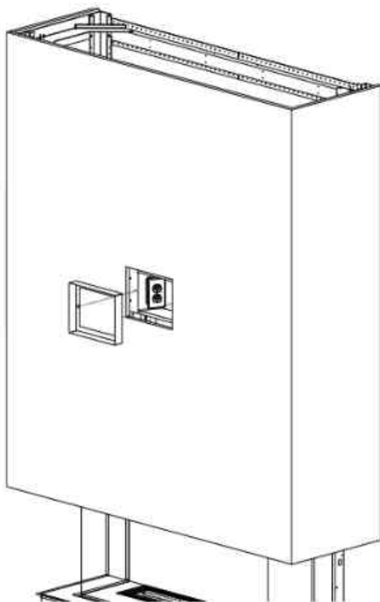
Install trim with 2 screws
