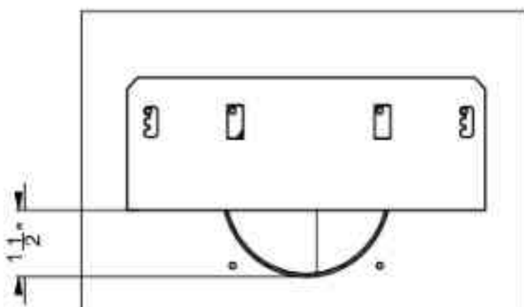
Set 3 (Vent restrictor at 1.5")
