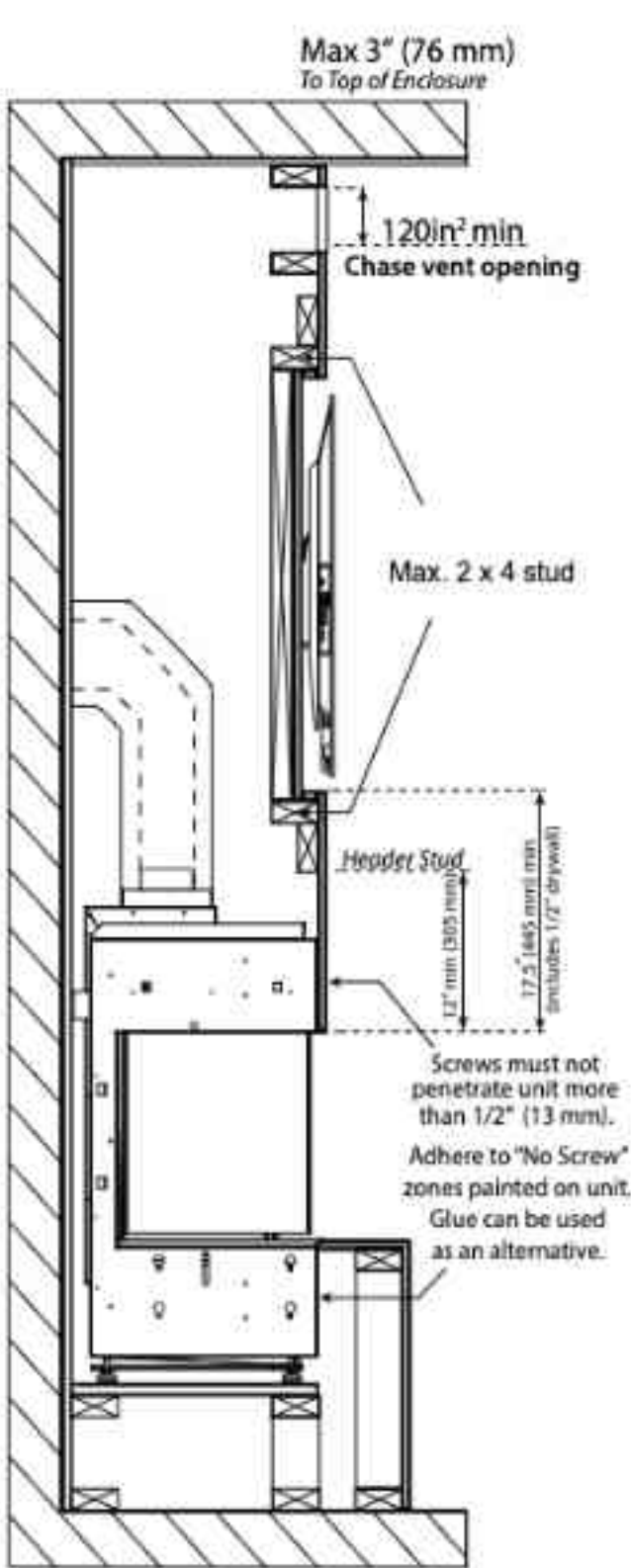
Flush wall TV recess using 1/2" (13 mm) drywall
