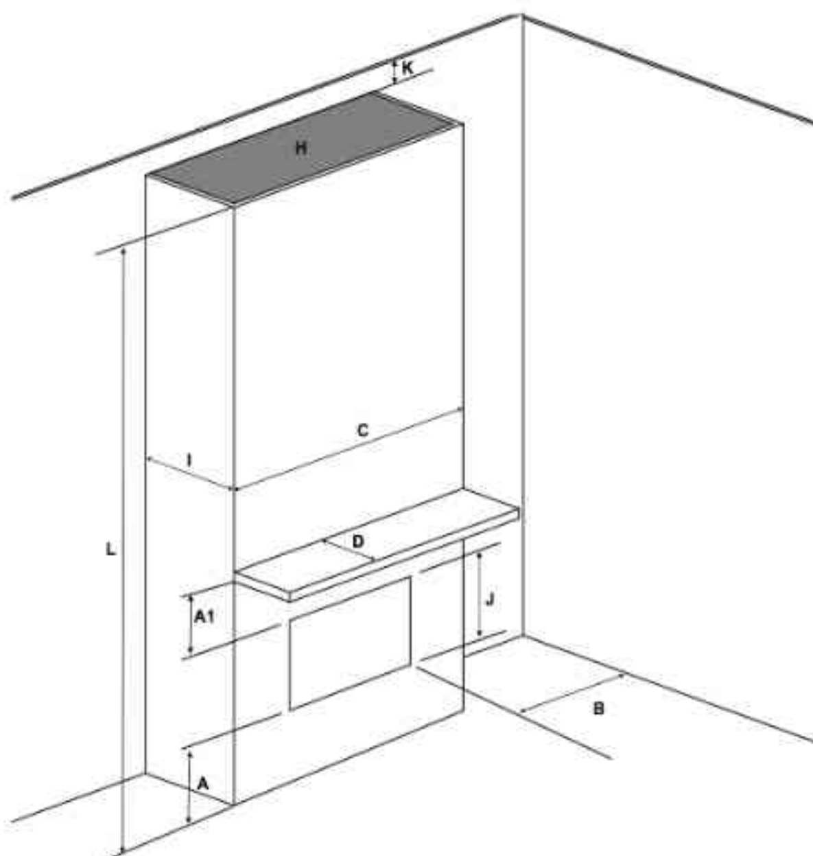
Floor to ceiling with top ventilation opening
