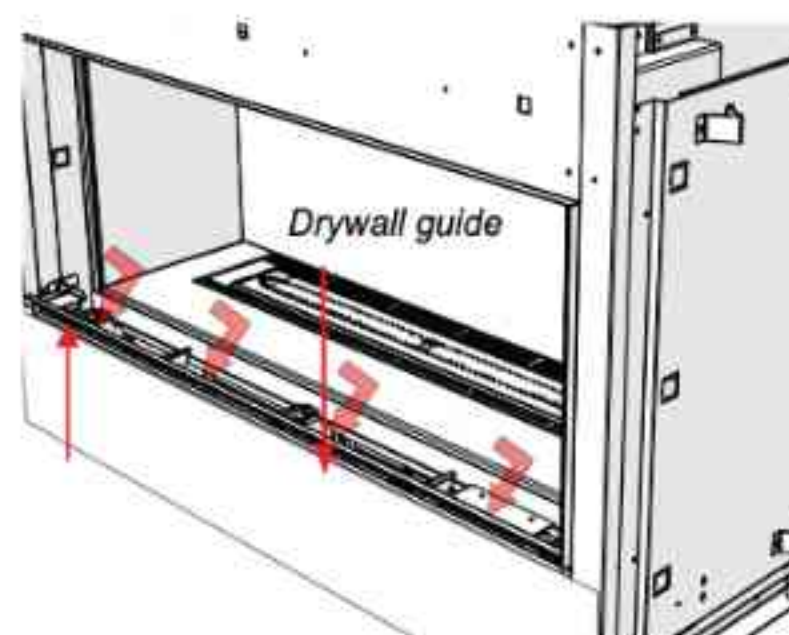
Diagram 1 - Loosen 4 screws and lift off lower drywall guide
