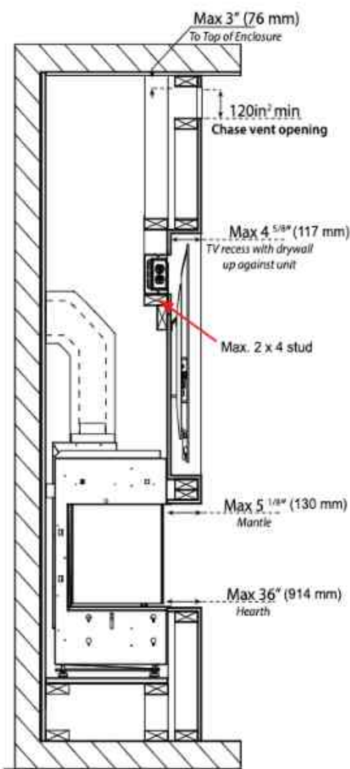
4 5/8" (117 mm) maximum TV recess using 1/2" (13 mm) drywall
