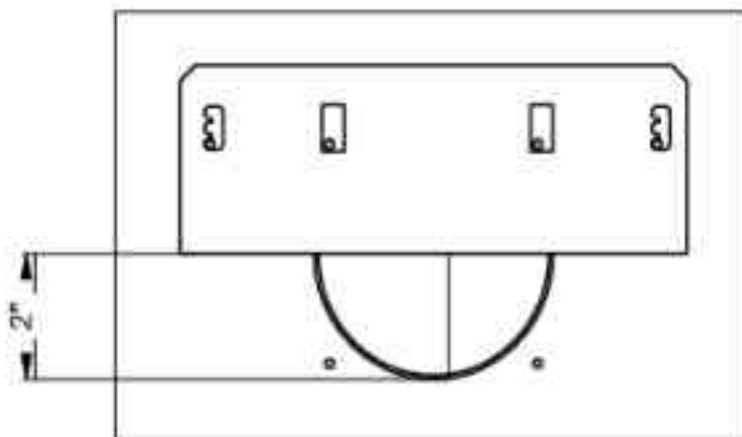
Set 1 (Vent restrictor at 2")
