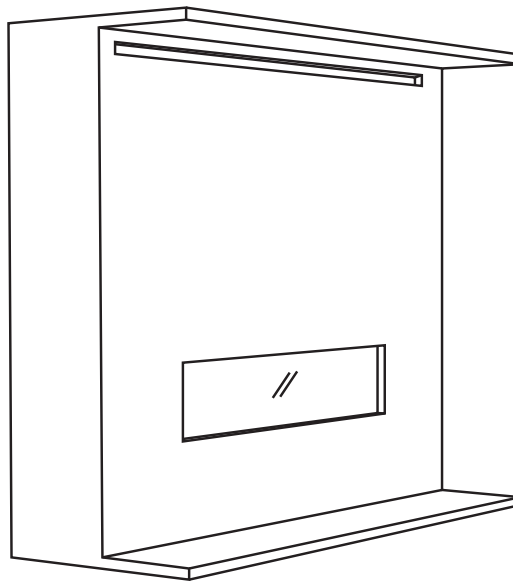
Custom chase vent Example dimensions: 2.5"x 48" (64 mm x 1219 mm) (120in 2 )
