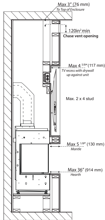
4 5/8" (117 mm) maximum TV recess using 1/2" (13 mm) drywall CB40E shown
