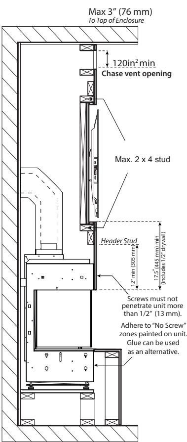
Flush wall TV recess using 1/2" (13 mm) drywall CB40E shown
