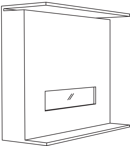
Reveal at the chase top Example dimensions: 2"x 60" (51 mm x 1524 mm) (120in 2 )
