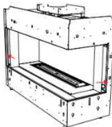
Outer side panel install
