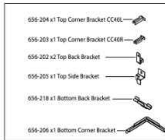
Glass Panel Parts Layout
