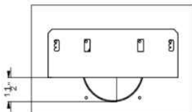
Set 3 (Vent restrictor at 1.5")
