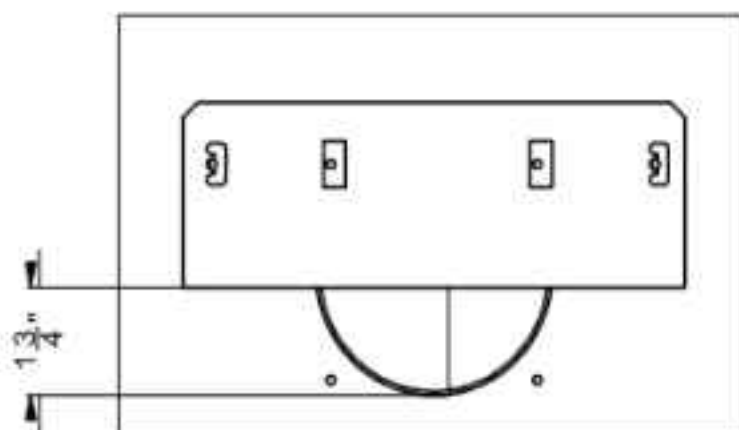
Set 2 (Vent restrictor at 1.75")
