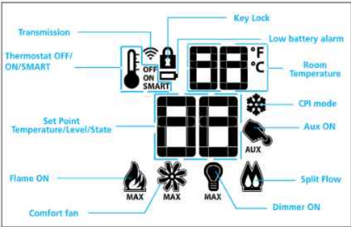
Figure 2: Transmitter LCD Display
