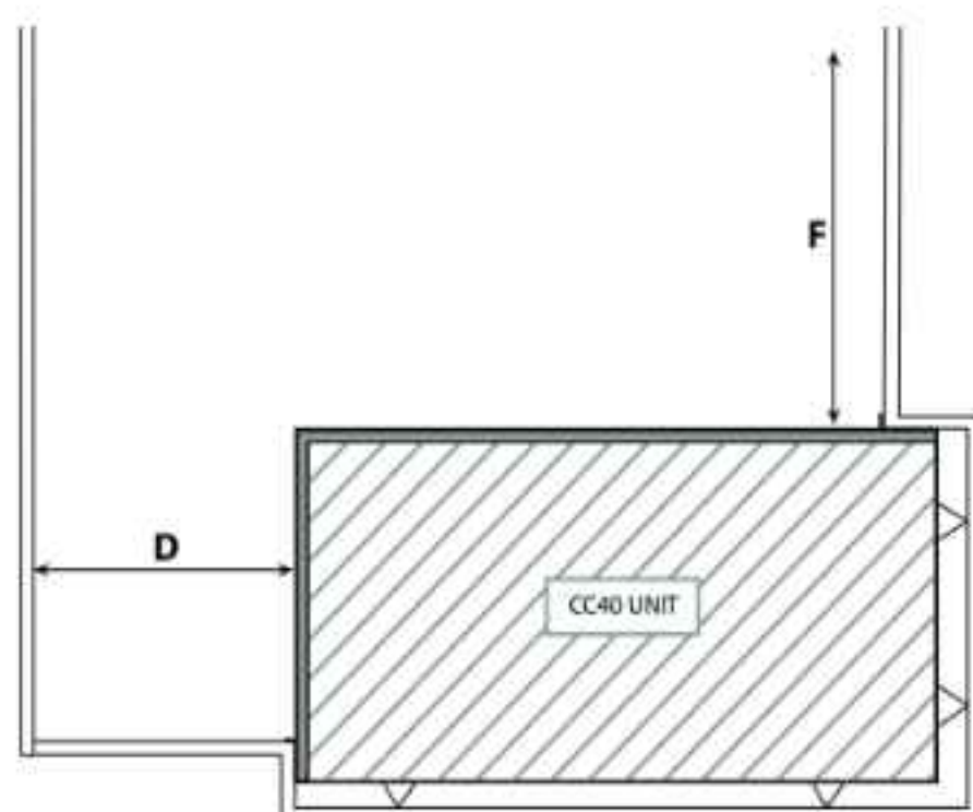
Top View Alcove
