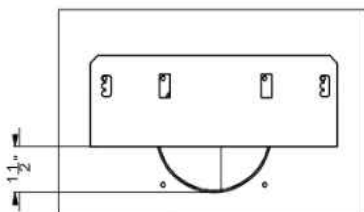
Set 3 (Vent restrictor at 1.5")
