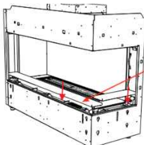
Outer base panel install
