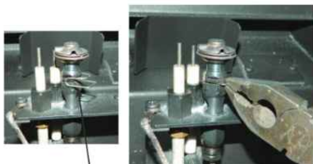
Pilot retainer clip
