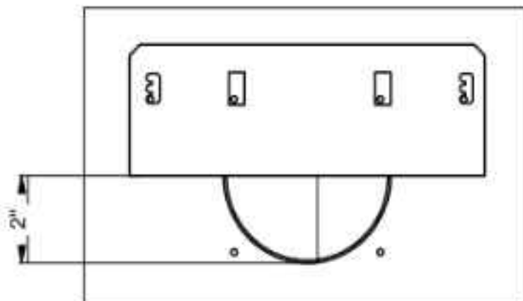
Set 1 (Vent restrictor at 2")
