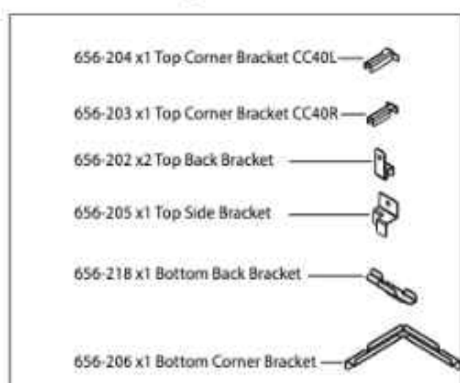
Glass Panel Parts Layout
