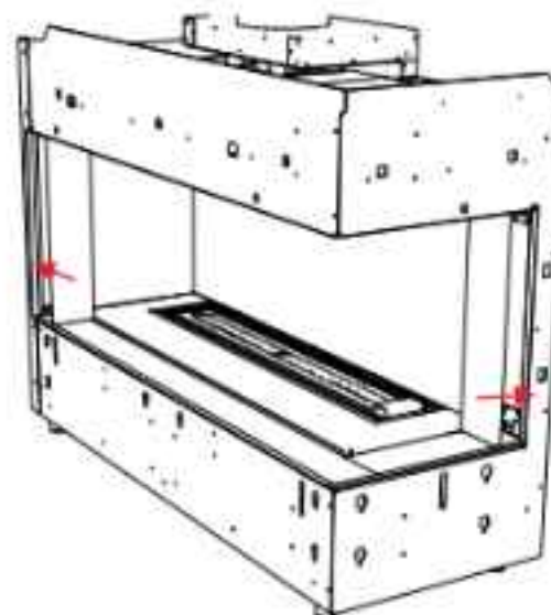
Outer side panel install
