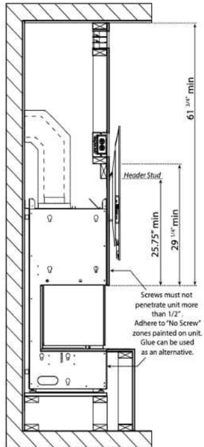
Flush wall TV install using 1/2" (13 mm) drywall.
