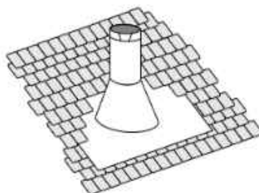
Diagram 4: The upper half of the flashing is installed under the roofing material and not nailed down until the chimney is installed. This allows for small adjustments.
