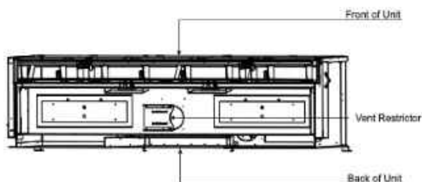
Cross section showing the ceiling of the firebox from the inside
