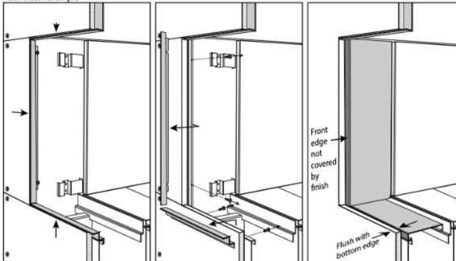
Flush Install Example
