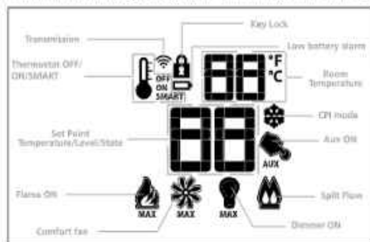
Figure 1: Transmitter LCD Display
