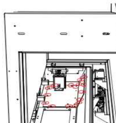
Remove 16 screws securing valve tray
