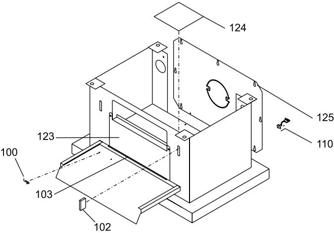
PEDESTAL (OPTIONAL)
