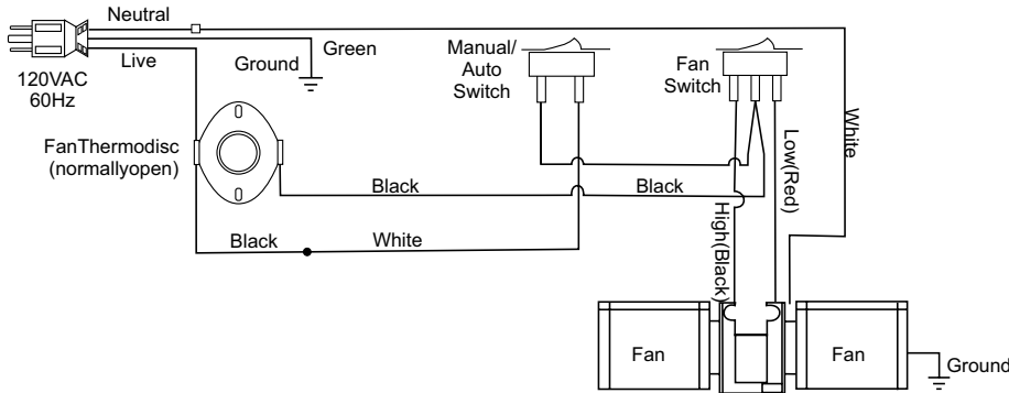
Blower/Fan Wiring Diagram
