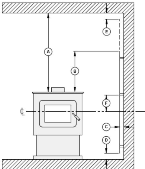
Figure 32: Heat shield clearances
