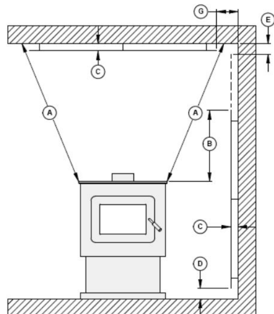
Figure 33: Heat shield clearances
