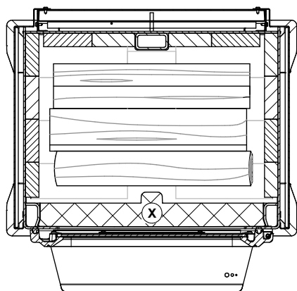
Figure 19: Position of the bottom pieces (High burn)
