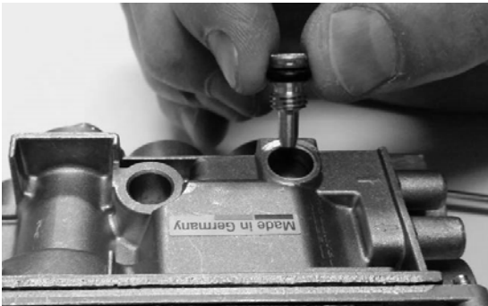
Figure 15 – NG Low Pressure Screw Insertion
