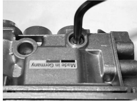
Figure 17 – Tighten NG Low Pressure Orifice
