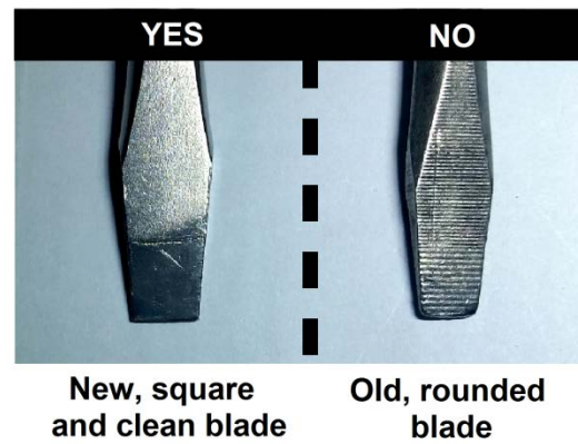
Figure 8 – Appropriate Bit Shape
